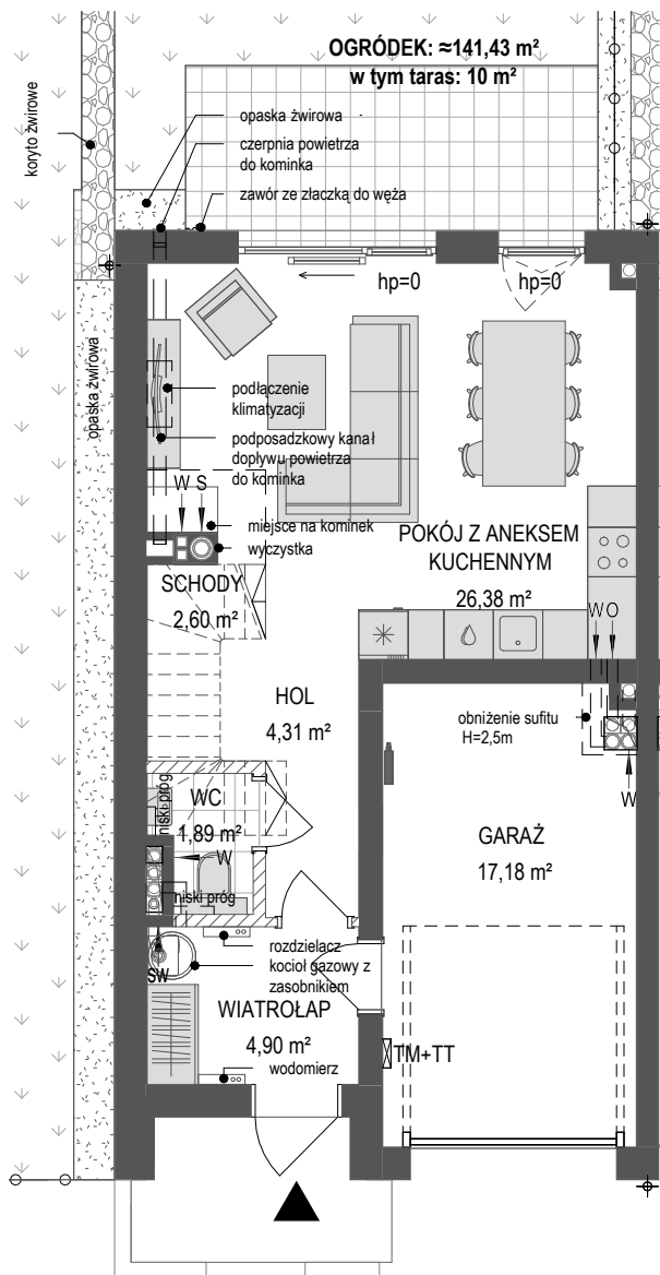
PARTER 57,26 m 2
